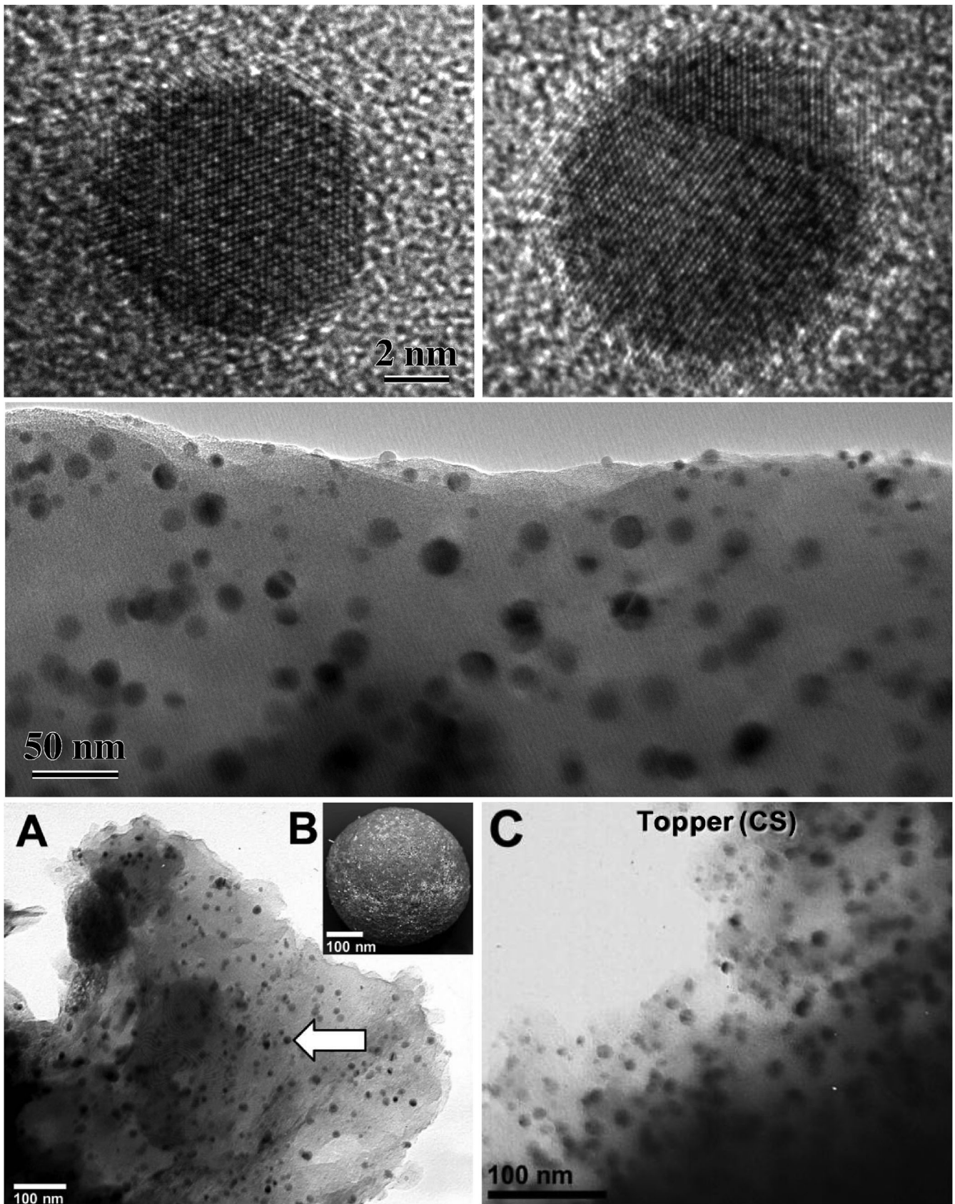
Figure 9. High-resolution TEM lattice images (top row) and bright-field (BF) TEM image of nanocrystals embedded within amorphous fragments (middle row) obtained from finely crushed carbon spherules collected from Arlington Canyon YDB sediments (AC-003). Many of the nanocrystals exhibit twinning, particularly \Sigma=3 twin boundaries or occasionally \Sigma=9 twin boundaries when successive \Sigma=3 twin domains impinge on one another (e.g. see Luyten et al. , 1992; Daulton et al. , 2003), characteristic of face centered cubic structures. Shown in the bottom row are fig. 13 (part A) and fig. 6 (part C) from Kinzie et al. (2014); their respective figure captions state, ‘carbon spherules from Gainey, Michigan (Younger Dryas Boundary [YDB]: 3933 ppb at 30 cm below surface [cmbs]’ and ‘nanodiamonds (NDs) in carbon spherules. (CS) ... n-Diamond from Topper, South Carolina (YDB: 108 ppb at 60 cmbs)’.
