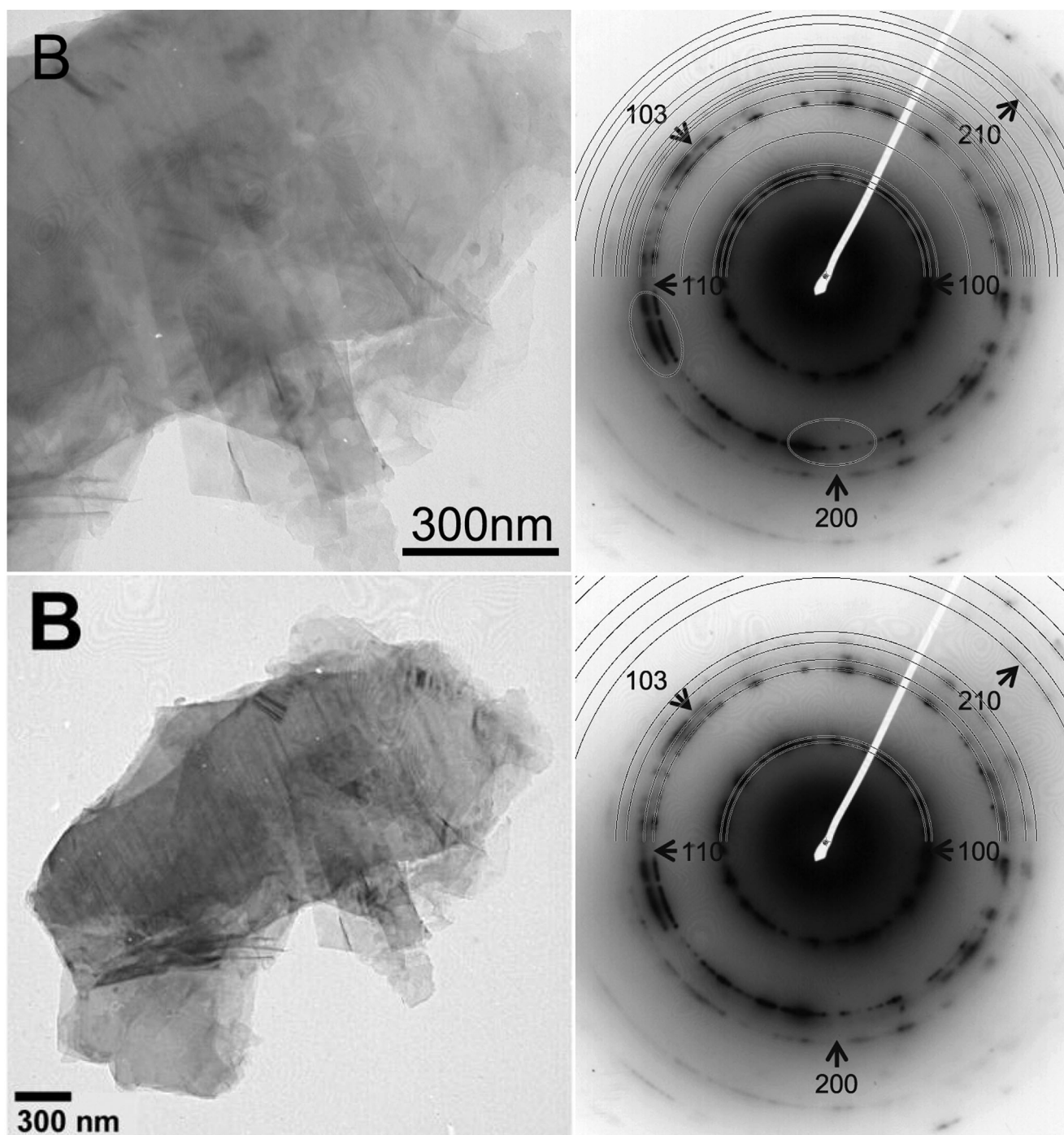
Figure 4. Shown in top row is fig. S2 (part B) of Kennett et al. (2009b); its figure caption states, '(B) cluster of lonsdaleite crystals and associated diffraction pattern from 4.59–4.64m(AC#348)'. We modified the diffraction pattern from the original published by Kennett et al. (2009b) by inverting its contrast to aid in visual clarity and by superimposing additional annotations on the pattern. In right of top row, ovals were superimposed to demonstrate the azimuthal asymmetry of the diffraction pattern and the presence of additional partial diffraction rings. Half circles were superimposed to illustrate the predicted reflections for lonsdaleite. The scale of the diffraction pattern was calibrated assuming that the ring labeled (110) by Kennett et al. (2009b) corresponds to the (110) reflection of lonsdaleite. Note that there are many missing lonsdaleite reflections. Left of bottom row is fig. 15 (part B) of Kinzie et al. (2014); its figure caption states, 'Younger Dryas Boundary lonsdaleite-like crystal'. This is the same grain shown in Kennett et al. (2009b). Shown at right of the bottom row is the diffraction pattern of Kennett et al. (2009b) with half circles superimposed to illustrate the predicted reflections for a homogeneous mixture of graphene and graphane where the \langle 100 \rangle d -spacing in graphane is contracted by a factor of 1.054 from that of graphene (Daulton et al. , 2010). The scale of the diffraction pattern was calibrated assuming the ring labeled (110) by Kennett et al. (2009b) corresponds to the (100) reflection of graphane. Consistent with this diffraction pattern, disordered graphite could be present and predominantly oriented with its [001] crystallographic axis in the electron beam direction. As such, the high-resolution lattice image published for this grain (fig. 16, Kinzie et al. , 2014) is consistent with a [001] zone axis of graphitic/graphene structure. Similarly, the diffraction pattern identified as lonsdaleite by Redmond and Tankersley (2011) is consistent with [001] graphite.
