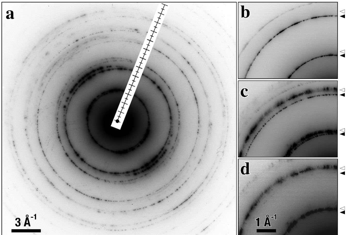
Figure 5. Typical electron diffraction pattern from aggregates of polycrystalline graphene/graphane recovered from sediments exhibits (a) azimuthally asymmetric electron diffraction rings indicative of texturing of two phases (Daulton et al. , 2010). Different regions within the same aggregate exhibit diffraction rings from (b) only graphene (solid triangles), (c) both graphene and graphane, or (d) only graphane (open triangles). To aid visual clarity, the diffraction patterns are displayed in reverse contrast.
