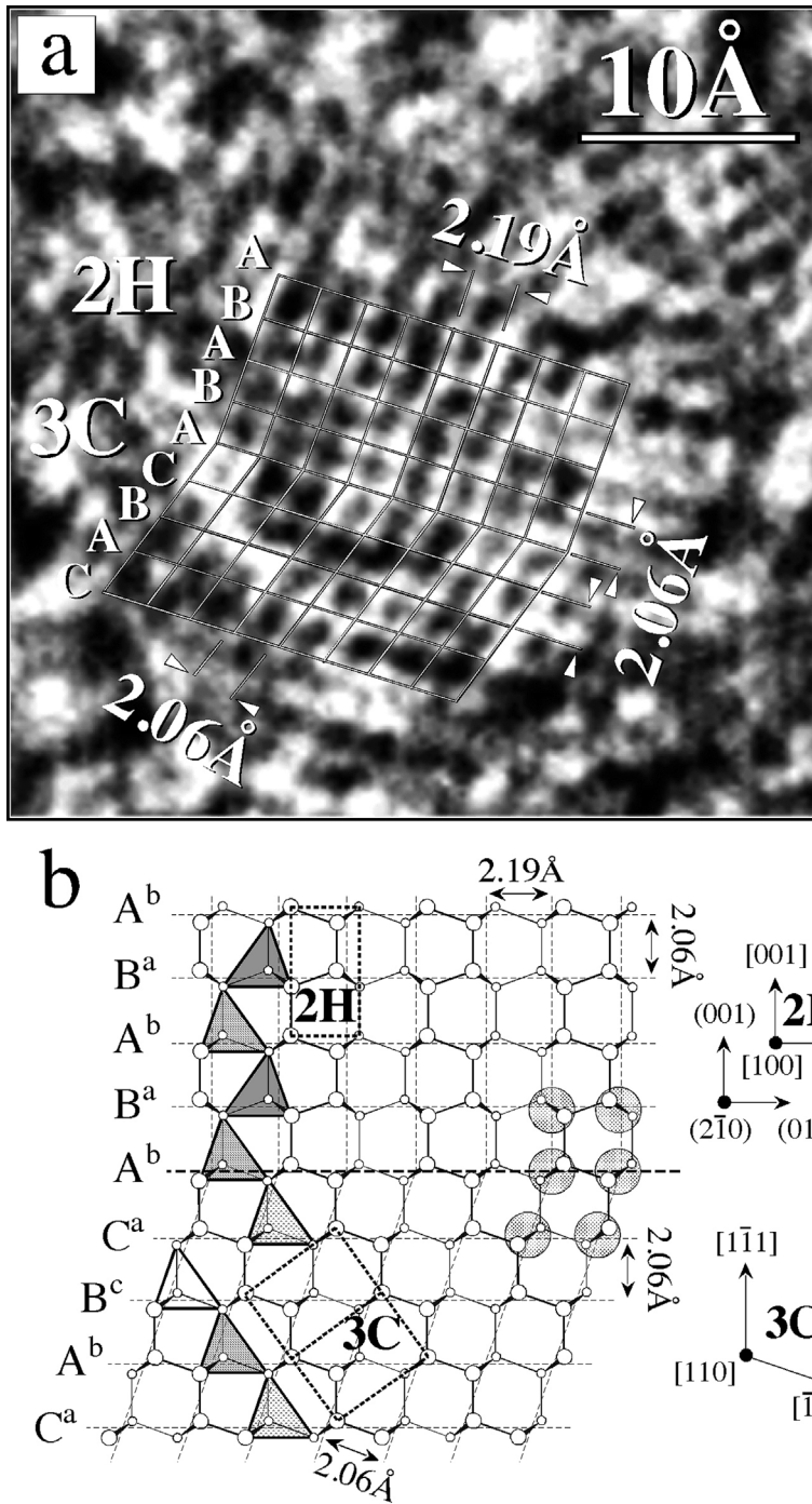
Figure 1. (a) An HR-TEM lattice image of a nanocrystal from the Allende meteorite acid-dissolution residue. The nanocrystal exhibits a homoepitaxial interface between two crystal lattices that is consistent with the (b) 3C cubic diamond and 2H lonsdaleite atomic structure (figure adapted from Daulton et al. , 1996). The grain displays one domain with close packed tetrahedral planes stacked in the (A^b)(B^a)(C^c) \dots sequence defining the 3C structure and a second domain stacked in the (A^b)(B^a) \dots sequence defining the 2H structure. Through-focus HR-TEM imaging (not shown) is consistent with these atomic structures. Furthermore, because this grain exhibits a homoepitaxial interface of two crystal structures, the possible pairs of candidate phases that comprise the grain are significantly limited. (c) Atomic models of the six unique (fundamental) bilayer planes ( A^b , A^c , B^a , B^c , C^a and C^b ) in diamond (top), that comprise stacked tetrahedral planes (depicted normal to stacking direction shown at bottom). The two basic stacking arrangements, (X^Z)(Y^Z) and (X^Z)(Y^Z) where X , Y and Z are all different, form planes of vertex-sharing antiparallel and parallel tetrahedra, respectively.
