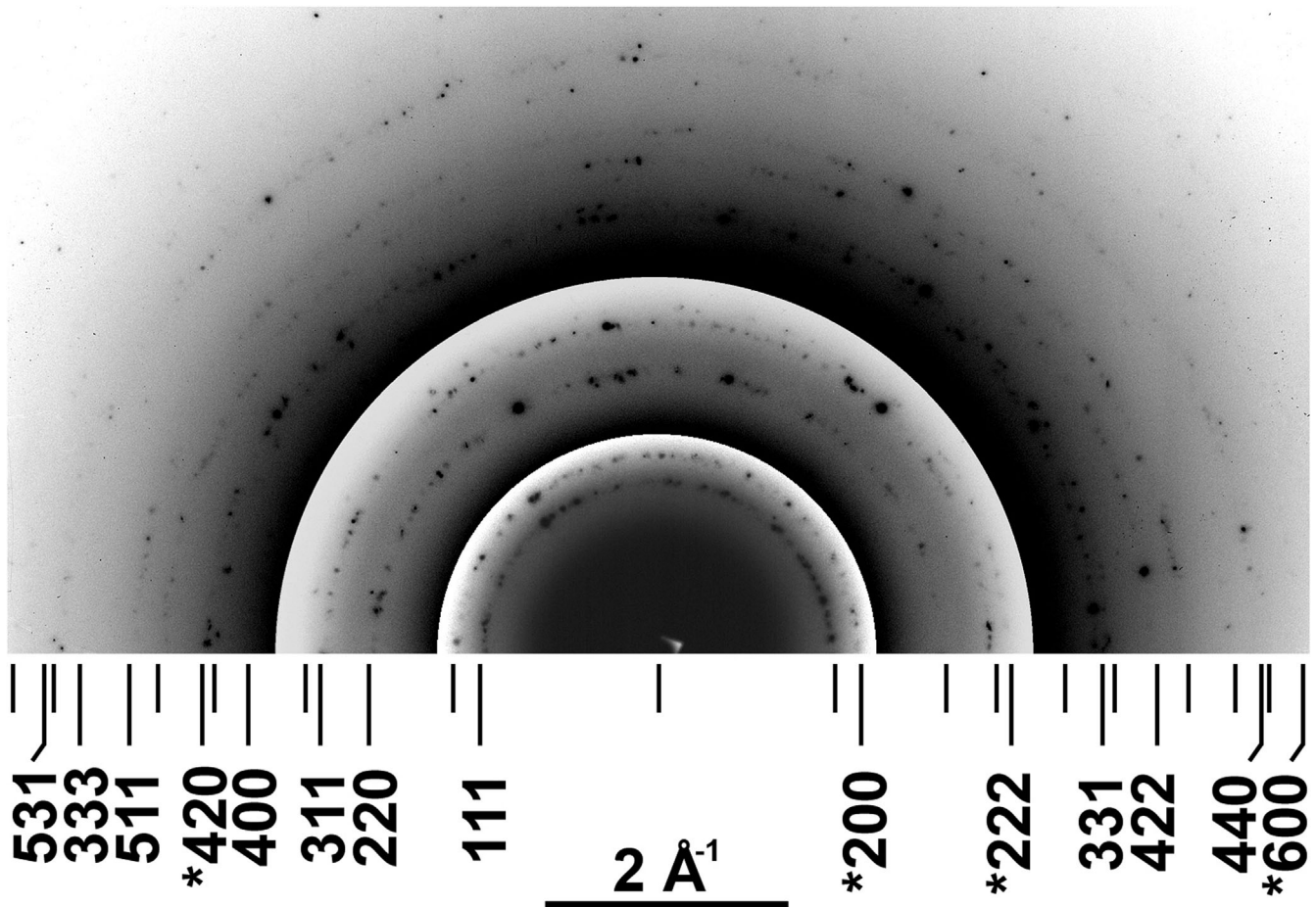
Figure 10. Representative diffraction pattern from amorphous grains obtained from finely crushed carbon spherules collected from Arlington Canyon YDB sediments (AC-003) that contain nanocrystals (see Fig. 9, middle row). The diffraction pattern is displayed in reversed contrast and three different electron exposures are superimposed to cover the large dynamic range of the Bragg intensities. The diffraction lines of cubic diamond (along with the kinematically forbidden diamond reflections denoted by *) are shown.
