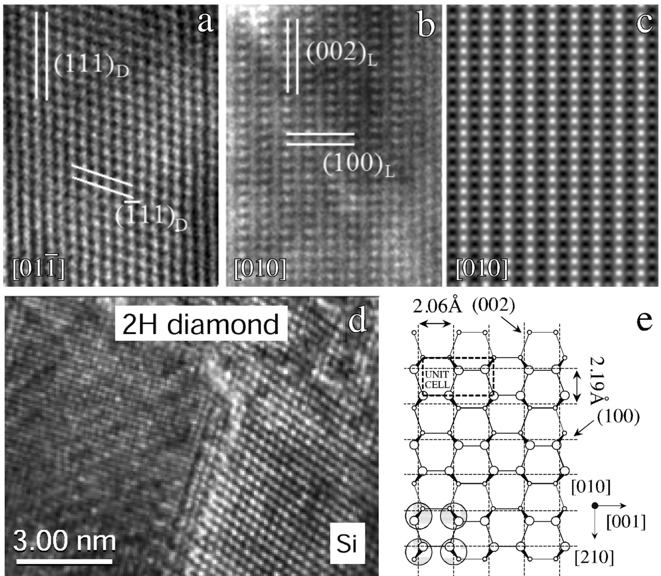
Figure 2. HR-TEM images of well-ordered (a) [01\bar{1}] zone of cubic diamond and (b) [010] zone of lonsdaleite from products of thermobaric high-pressure, high-temperature treatment of graphite. (c) Calculated HR-TEM image of lonsdaleite for [010] zone axis (figure adapted from Kulnitskiy et al. , 2013). (d) HR-TEM image of diamond grown on (100) -oriented Si held at 600 or 700 °C by bombardment with 80- or 200-eV ions from a (\text{CH}_4 or \text{C}_2\text{H}_2)/\text{Ar}/\text{H}_2 -fed Kaufmann source (figure adapted from Lifshitz et al. , 2001). (e) Schematic atomic model of lonsdaleite projected along the [010] zone axis.
