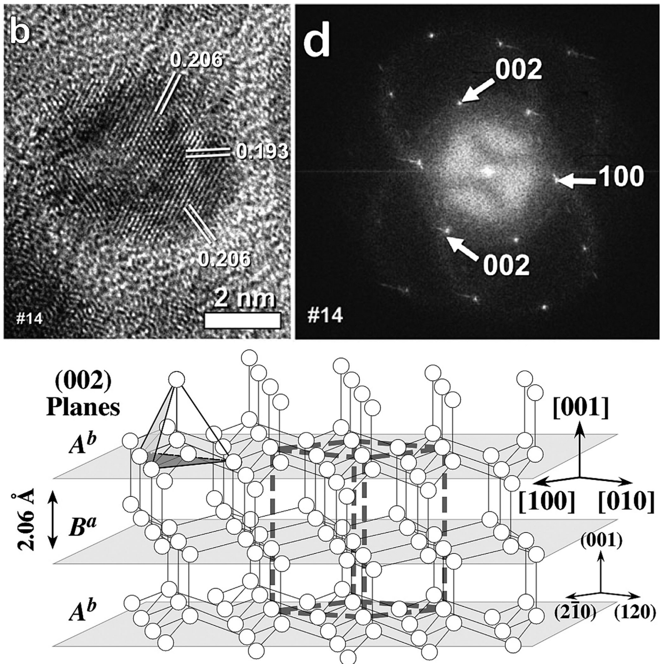
Figure 3. Shown in top row figure 6 part b and part d of Kurbatov et al. (2010); its figure caption states, 'Lonsdaleite analyses. (b) HR-TEM image showing characteristic lonsdaleite lattice spacings. (d) Fast Fourier transform (FFT) of lonsdaleite ND crystal. All values (Miller indices) are consistent with each other and with the published lattice spacings for lonsdaleite as shown in Table 3. Sample numbers, as referenced in Table 2, are shown in the lower left of each image.' Shown at the bottom is a schematic of the atomic structure of lonsdaleite. In diamond, C atoms covalently bond to four other C atoms in a tetrahedral geometry. The {002} planes in the lonsdaleite structure contain the base of the C tetrahedra that are stacked in the structure. The set of {002} planes are oriented edge-on only in [hk0] zone axes projections, and high-resolution lattice images of [hk0] zone axes display only one set of {002} planes, contrary to the nanocrystal shown by Kurbatov et al. (2010).
