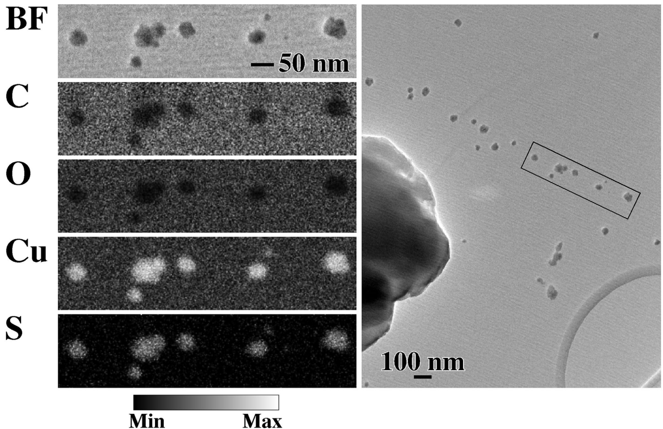
Figure 12. Top: bright-field (BF) image of nanocrystals from finely crushed carbon spherules collected from Arlington Canyon YDB sediments (AC-003). Below are STEM energy dispersive X-ray spectroscopy (EDXS) maps of relative elemental composition normalized to the sum of C, O, Cu and S contributions. C and O is associated with the support film and deficits in those elements occur in the maps where the nanocrystals are located due to the normalization of the elemental compositions to the sum of C, O, Cu and S contributions. If the nanocrystals contained C, excesses in C would be observed at the locations of the nanocrystals. The 256 greyscale look-up table (LUT) is linearly mapped between the minimum and maximum element composition for each map. (The elemental maps are published online in false color with a dynamic range of 1786 colors.)
