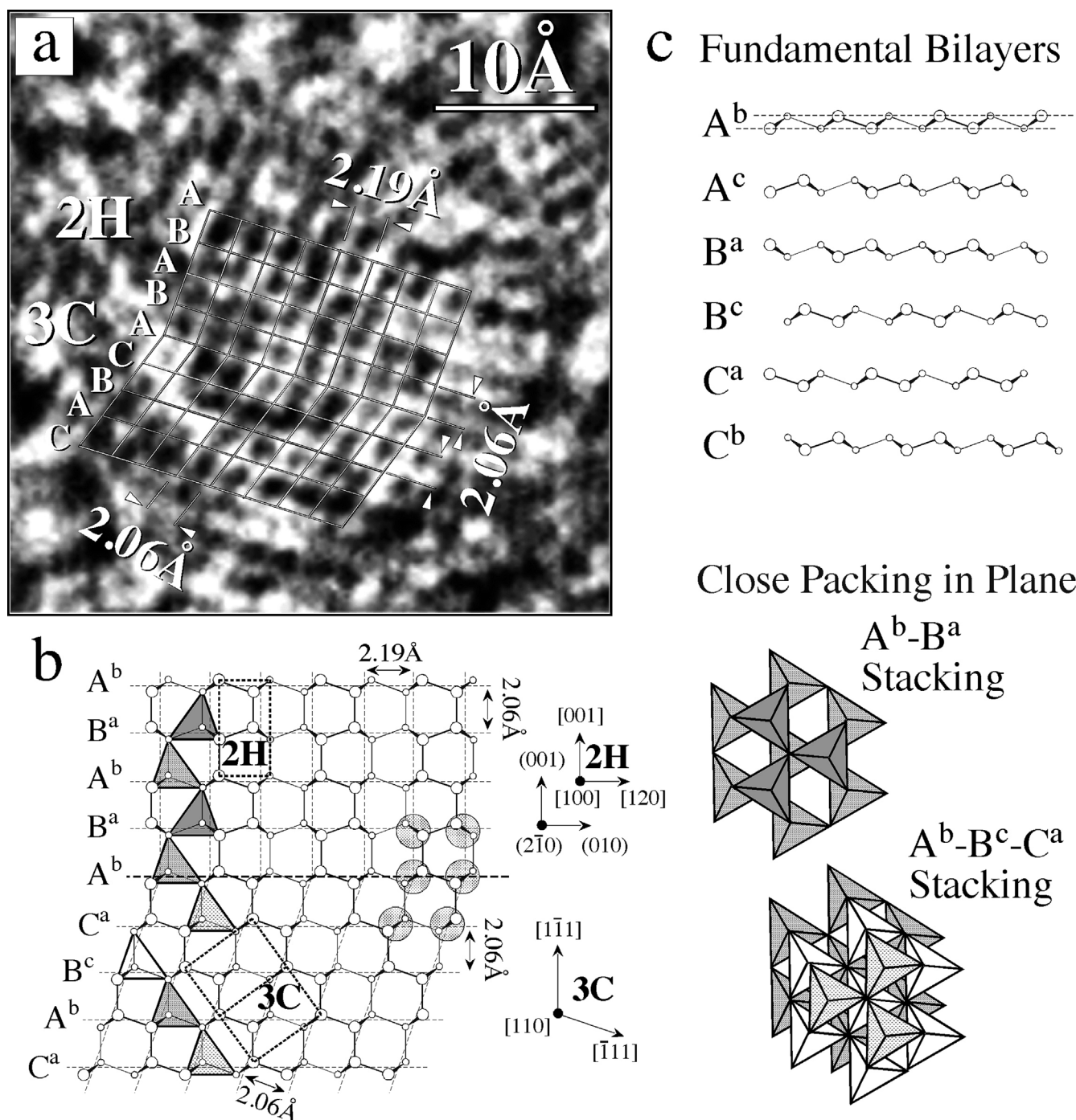
Figure 1. (a) An HR-TEM lattice image of a nanocrystal from the Allende meteorite acid-dissolution residue. The nanocrystal exhibits a homoepitaxial interface between two crystal lattices that is consistent with the (b) 3C cubic diamond and 2H lonsdaleite atomic structure (figure adapted from Daulton et al. , 1996). The grain displays one domain with close packed tetrahedral planes stacked in the (A^b)(B^a)(C^a) \dots sequence defining the 3C structure and a second domain stacked in the (A^b)(B^a) \dots sequence defining the 2H structure. Through-focus HR-TEM imaging (not shown) is consistent with these atomic structures. Furthermore, because this grain exhibits a homoepitaxial interface of two crystal structures, the possible pairs of candidate phases that comprise the grain are significantly limited. (c) Atomic models of the six unique (fundamental) bilayer planes ( A^b , A^c , B^a , B^c , C^a and C^b ) in diamond (top), that comprise stacked tetrahedral planes (depicted normal to stacking direction shown at bottom). The two basic stacking arrangements, (X^Z)(Y^Z) and (X^Z)(Y^Z) where X , Y and Z are all different, form planes of vertex-sharing antiparallel and parallel tetrahedra, respectively.
