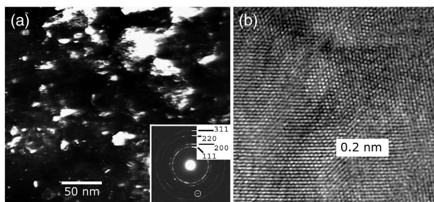
Fig. 6. (a) Dark field of a contiguous area of nanograins together with the corresponding SAED ring pattern including the used aperture. (b) HRTEM image of an area as seen in (a) and revealing several lattice defects and distorted zones.
