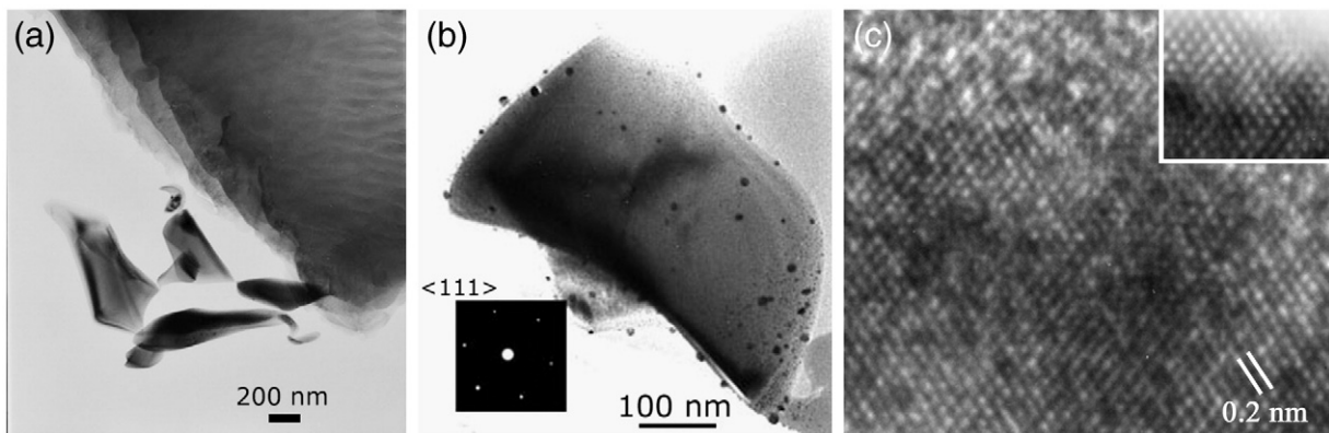
Fig. 8. Several examples of micrometer sized flake-shaped particles including the \langle 111 \rangle zone for the normal to the surface of the flake in (b). (c) HRTEM image of the edge of a microflake observed along a [110] zone including inset showing an edge dislocation.
