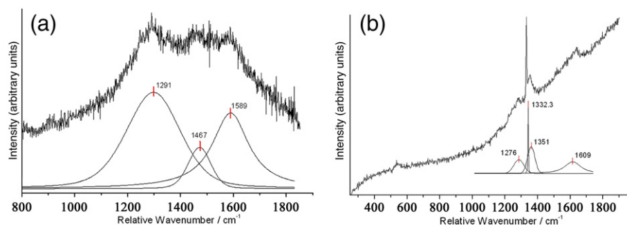
Fig. 11. (a) Typical Raman spectrum of a spherule interior showing amorphous carbon, distorted graphite and carbon atoms in spherical surroundings and (b) of a spherule showing a diamond peak at 1332.3 \text{cm}^{-1} .
